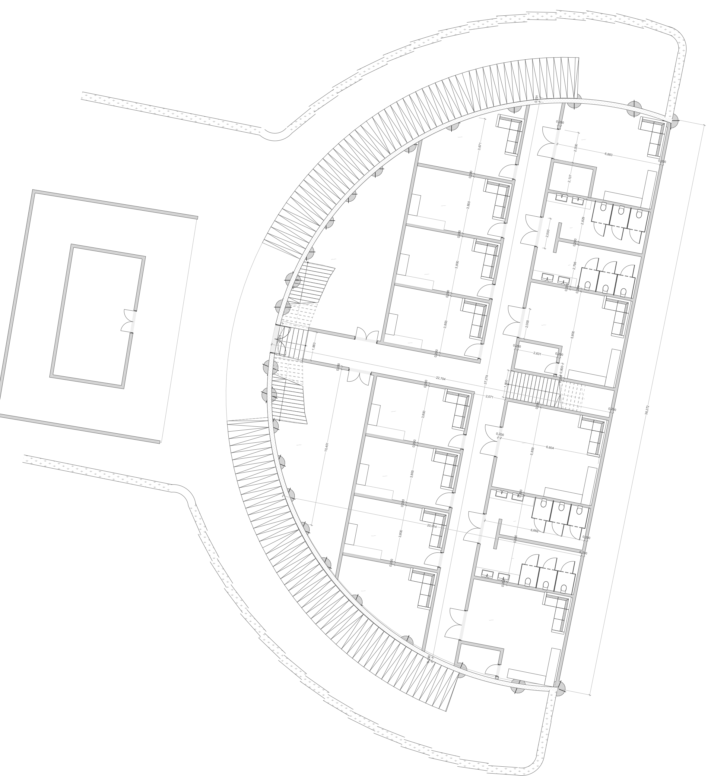
P04 CAMERINOS TARIMA 1 1:200
