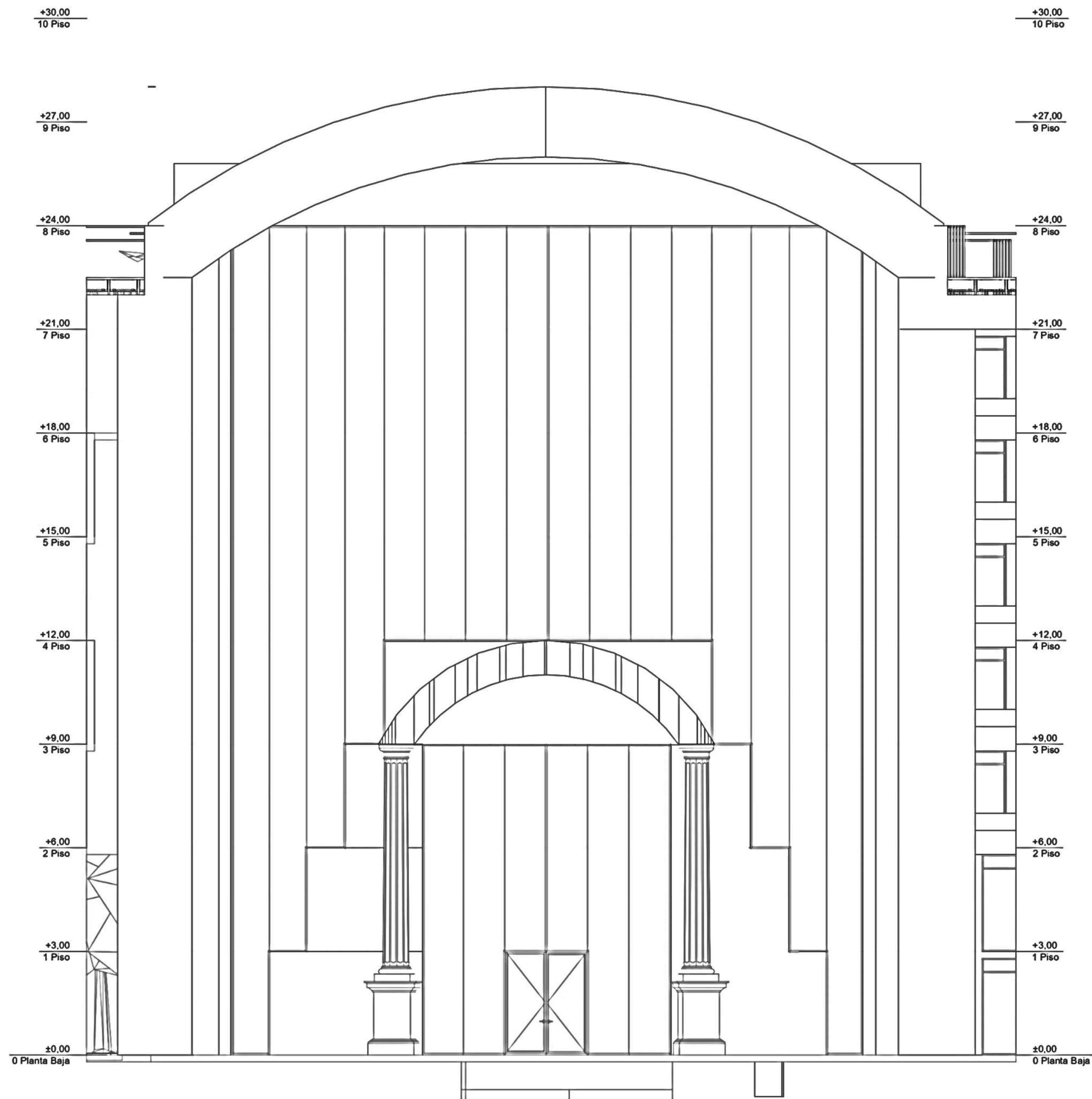
FACHADA PRINCIPAL ESC 1:100
