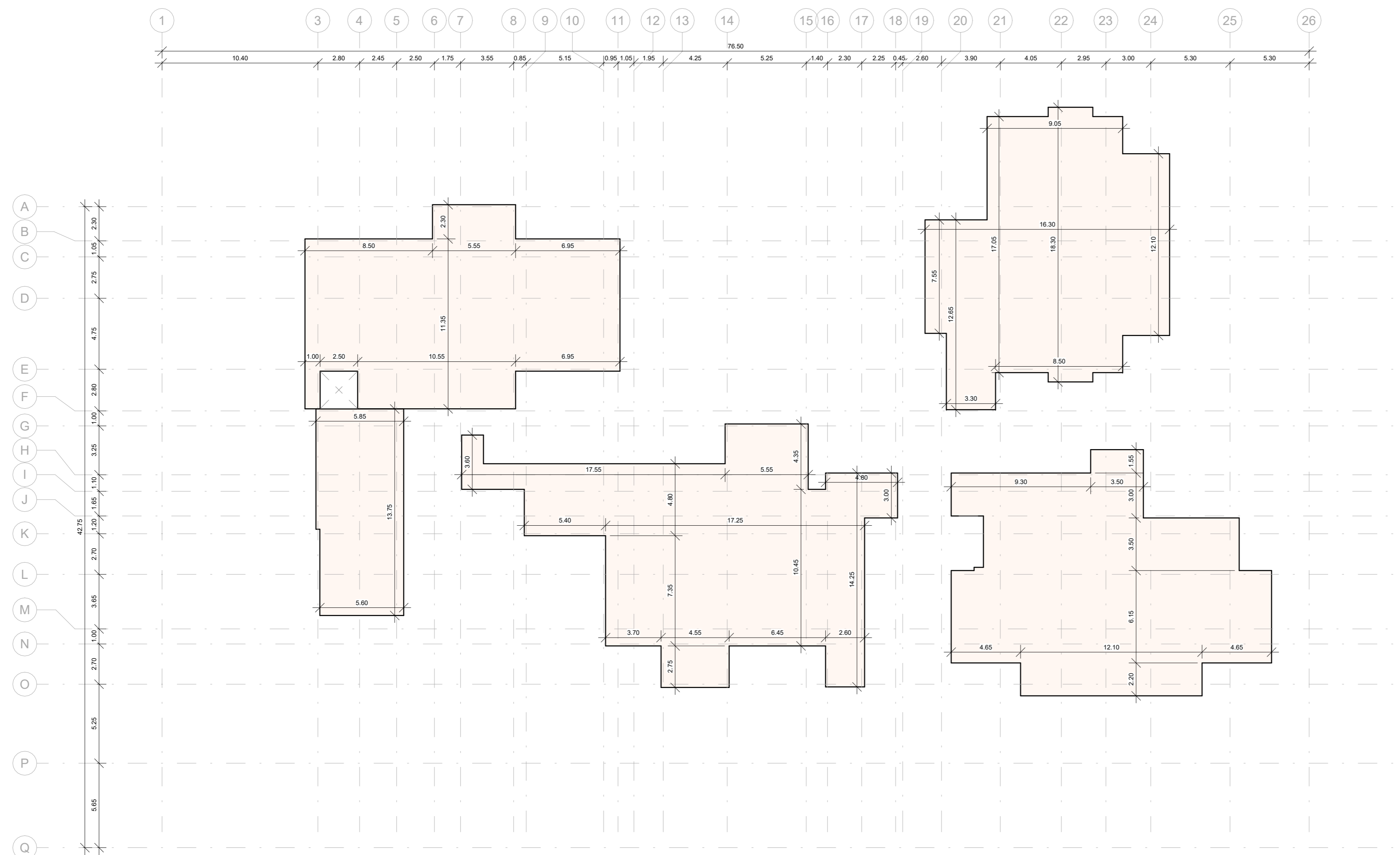
1 LEVEL 2.5 - PLACAS CLT 1 : 200
