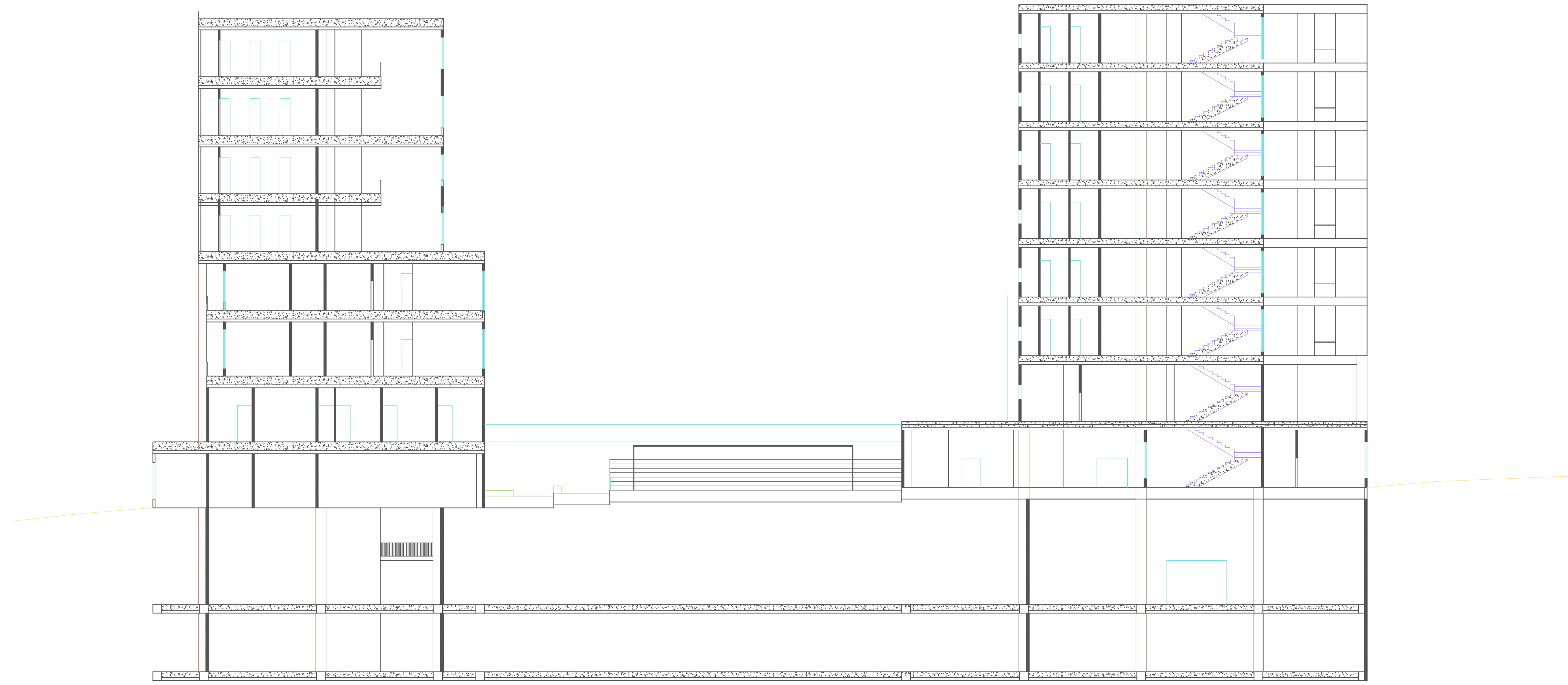
A CORTE VERTICAL C1 ESC: 1000/200
