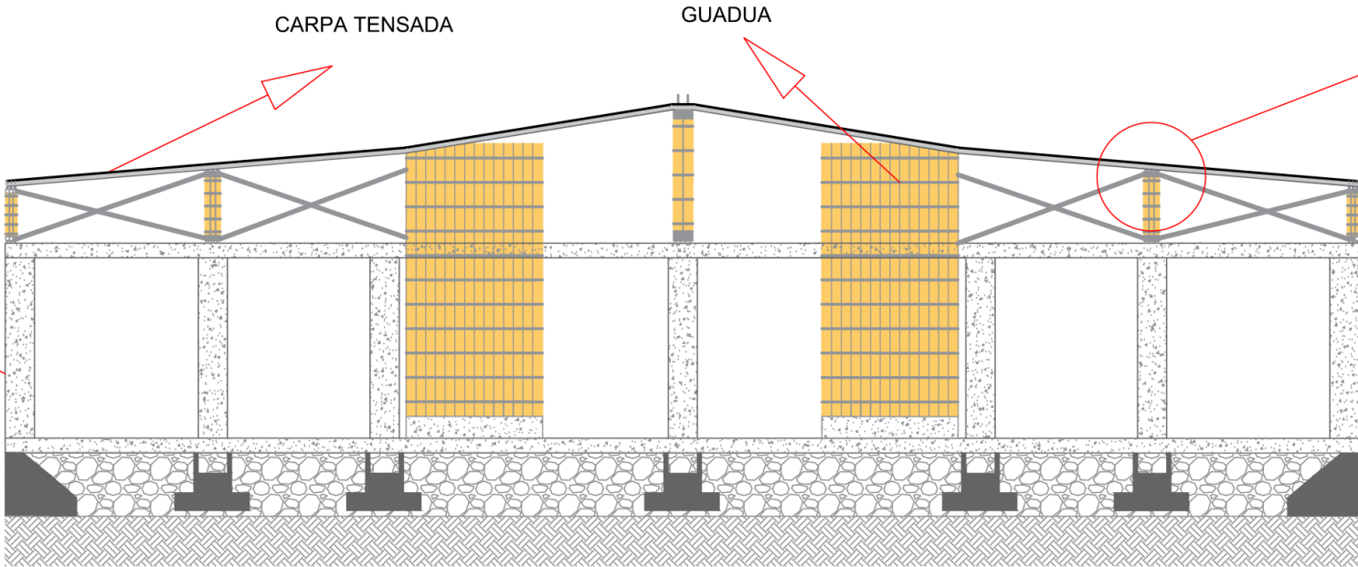
CORTE TRANSVERSAL AREA 556 MT2
