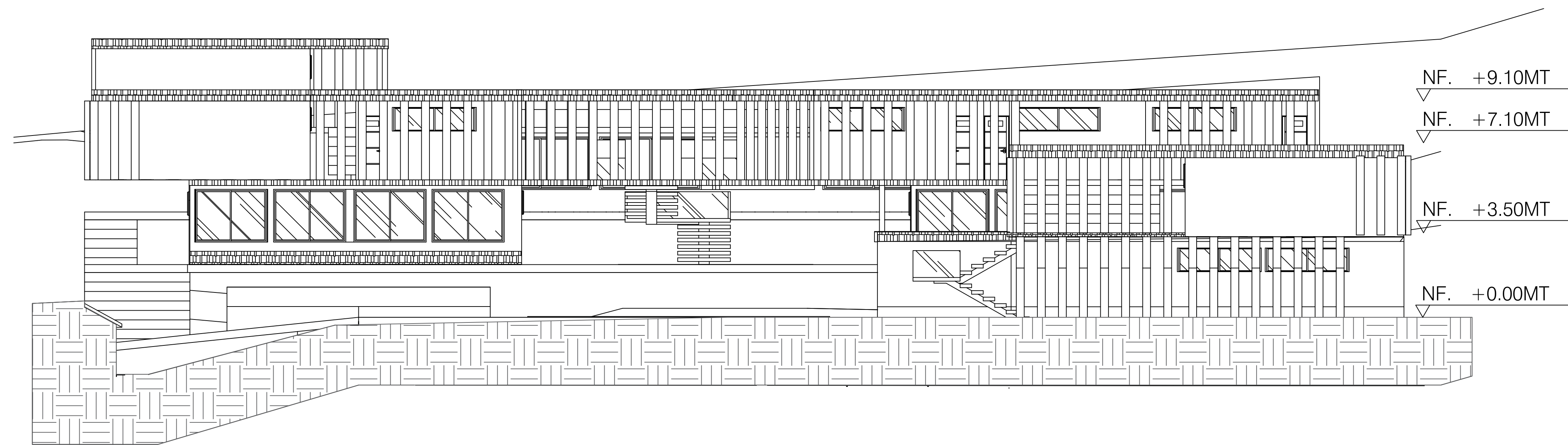
F FACHADA PRINCIPAL ESCALA 1:200
