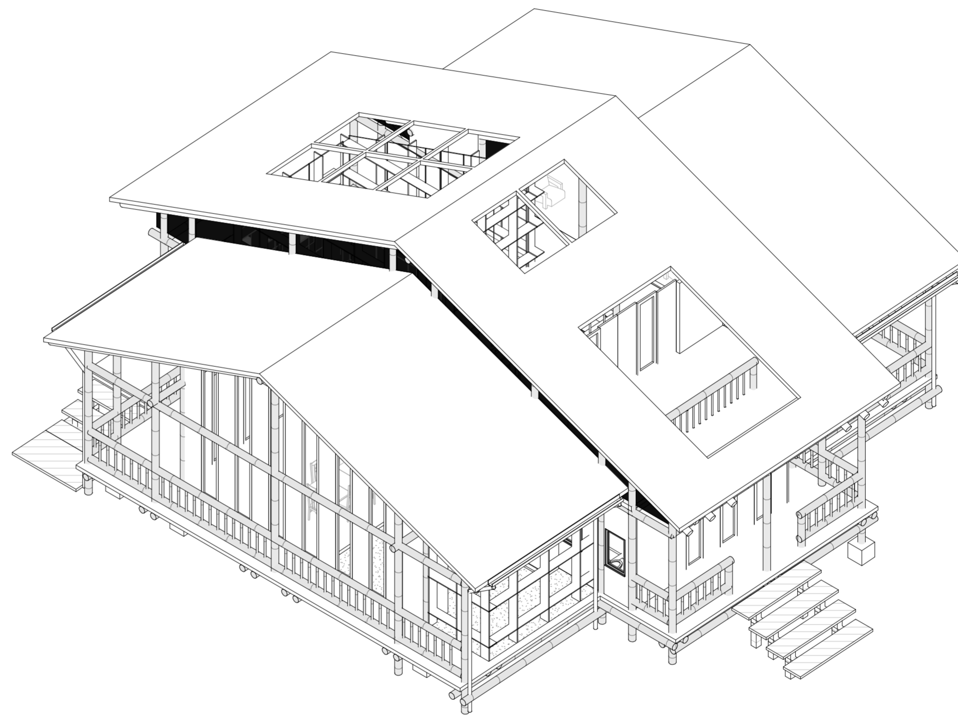
3 ISOMETRICO GENERAL
