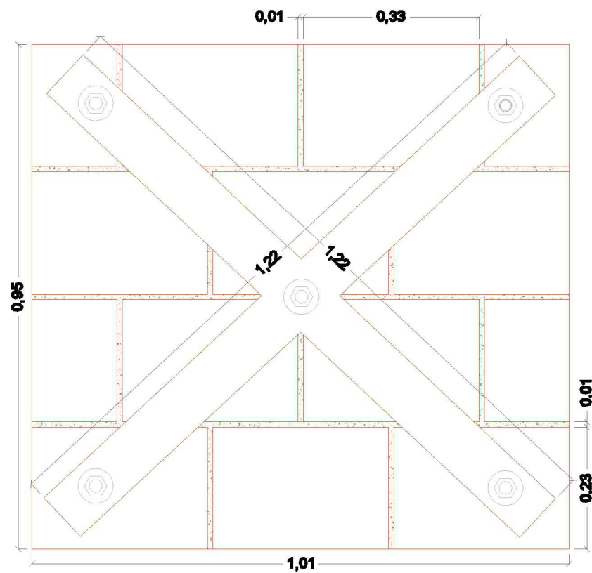
VISTA FRONTAL
